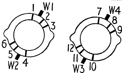
The switch banks of the 8321. Bank (1) is left and (2) right (see under-chassis diagram).
