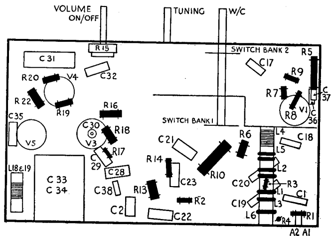
The switch banks of the 8321. Bank (1) is left and (2) right (see under-chassis diagram).
