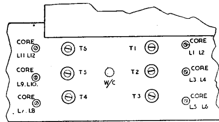
TRIMMER LAYOUT.
