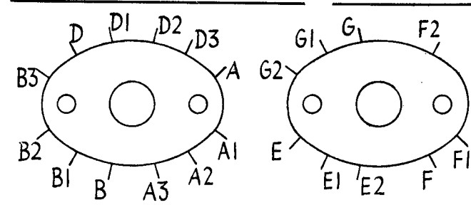
Left, is the switch arrangement employed in the Ekco AW70. The wiring table is given in col. 3 on the right.
